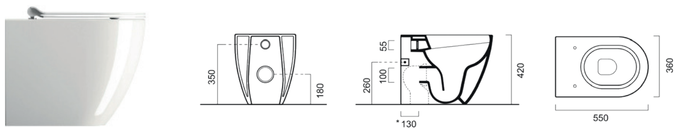
889011 WC PURA SWIRLFLUSH BIANCO LUCIDO 55X36 BACK TO WALL - SA273
