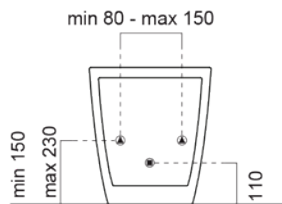
9862111 BIDET MODO SWIRLFLUSH 52X37 BACK TO WALL - SA271
